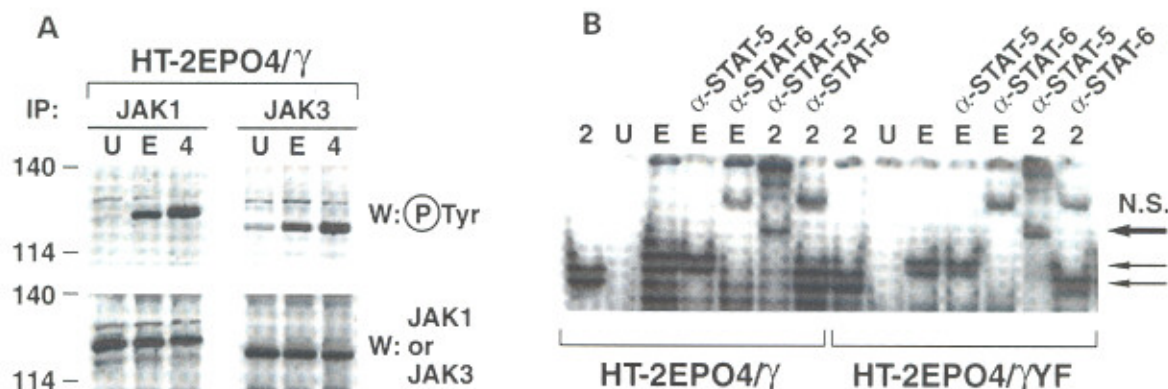
Fig. 1. The IL-4R \alpha - \gamma heterodimer mediates activation of the JAK-STAT pathway. (A) Lysates from HT-2EPO4/ \gamma cells unstimulated (U) or treated with EPO (E, 50 U/ml) or IL-4 (4, 50 U/ml) were subjected to serial immunoprecipitation with anti-JAK1 and anti-JAK3 antisera. Immunoblotting was performed with an anti-phosphotyrosine antibody (4G10). Blots were then stripped and re-probed with anti-JAK1 or anti-JAK3 antisera to verify even sample loading. (B) EMSA of nuclear extracts from HT-2EPO4/ \gamma and HT-2EPO4/ \gamma YF cells that were rested (U) or stimulated with IL-2 (2, 10 nM) or EPO (E, 50 U/ml). Competition was performed with the anti-STAT-5 and anti-STAT-6 antibodies. The lower two arrows highlight EPO-induced (top) and IL-2-induced (bottom) bands. The bold arrow indicates the complex supershifted by anti-STAT5 antibody. N.S., non-specific band.
