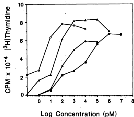
FIG. 1. Mitogenic dose-response of FDC-P1 cells to various growth factors. FDC-P1 cells were incubated for 36 hr in serum-free medium with various concentrations of IL-4 (●), IL-3 (○), insulin (■), or IGF-I (▲). [ ^3\text{H} ]Thymidine (0.5 \mu\text{Ci} per well) was added for 4 hr and samples were then collected by an automatic harvester. Results are expressed as counts per minute (cpm) in stimulated samples minus background cpm.
